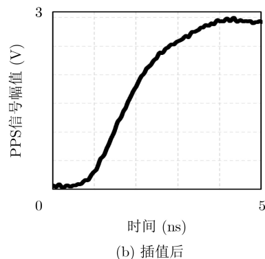
图8 GPS L1C/A频点GNSS模拟器校准
