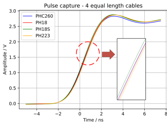
Figure 4. Pulses observed after passing through 1 m cables.
