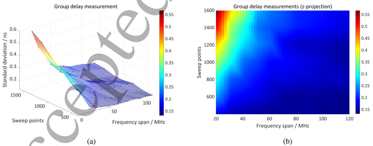
Figure 11. (a) Measurements of group delay during parameter traversal. The black dots represent the average mean values of 10 measurements taken under specific parameters, and the grid plot is derived by interpolation using the same method as in figure 10 to obtain a smoother distribution of the data. (b) The z-projections of the traversed results after interpolation. (c) Converted aperture-mean scatter plot of the measurements during parameter traversal.
