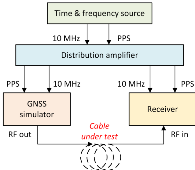
Figure 9. Scheme of the pseudorange simulation measurement.
