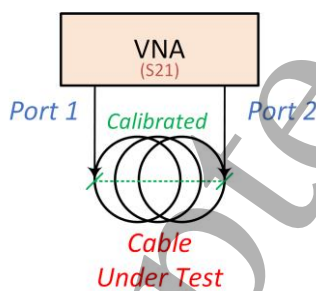
Figure 5. Schematic of the group delay measurement.
