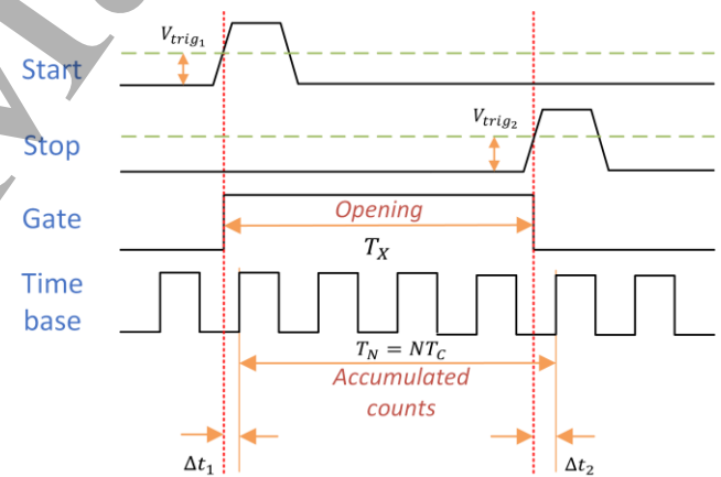
Figure 2. Simplified illustration of time interval measurement.
